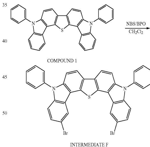
[Reaction Scheme 8]
