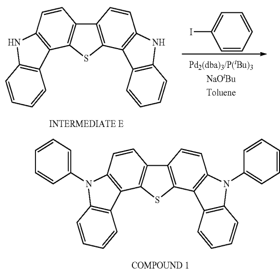
[Reaction Scheme 6]
