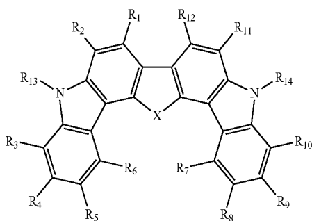
[Formula 1]
