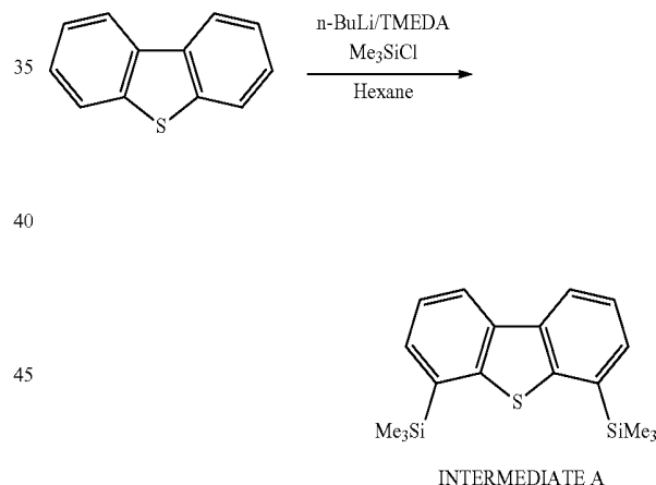
[Reaction Scheme 1]
