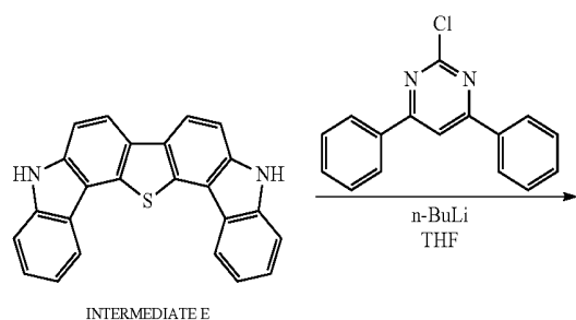
[Reaction Scheme 7]
